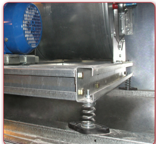
VIBRO AM APPLICATION IN CENTIFUGAL FAN
